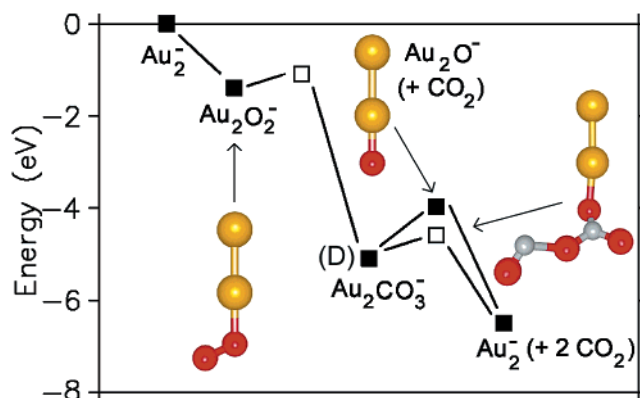
Figure 8. Energetics of the ER mechanism of the reaction where the carbonate species Au 2 CO 3 - (configuration D in Figure 6) is the metastable intermediate state. The open squares denote the reaction barriers. The first reaction barrier is associated with the insertion of CO into the O–O bond of Au 2 O 2 - (see structure on the left) leading to formation of Au 2 CO 3 - . Subsequently, two reaction paths are shown. One path involves thermal dissociation of the carbonate to produce Au 2 O - (see the structure shown at the top) which then reacts with CO(g) releasing another CO 2 molecule. The other path proceeds through an ER reaction of the carbonate with CO(g) and it results in the formation of two CO 2 molecules. The latter path involves a barrier of 0.5 eV, and the corresponding transition-state configuration is shown on the right.
